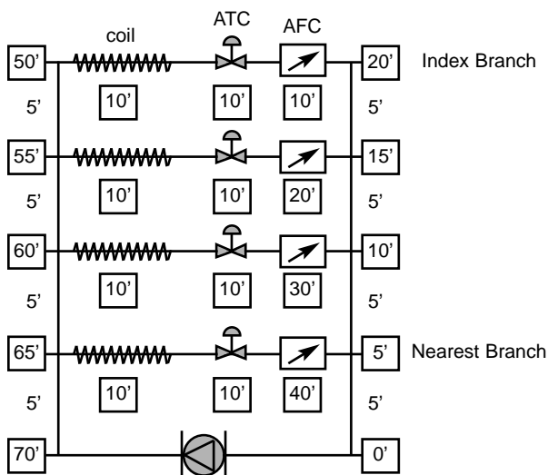
Example – Multiple Branch, Constant Speed System
